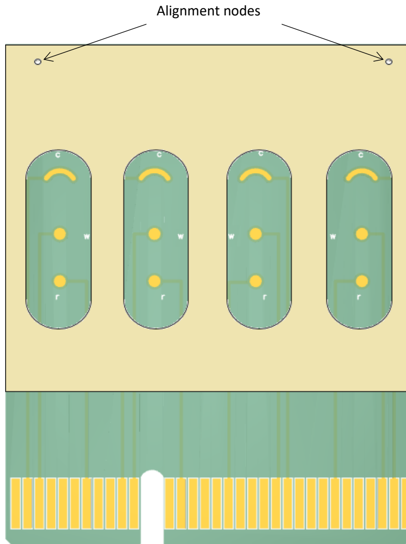
Figure 2: biotIP® SEP4, confinement mask fitting over the SEP1 electrode set.
